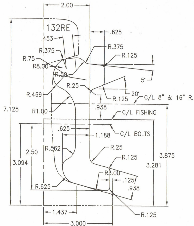
MICROALLOYED JOINT BAR PER AREMA PART 3 SEC 3.4 DTD 2005
